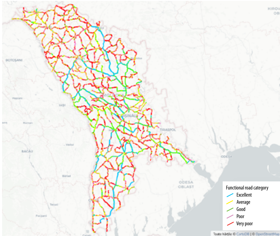
Figure 31 Moldova road roughness index map
