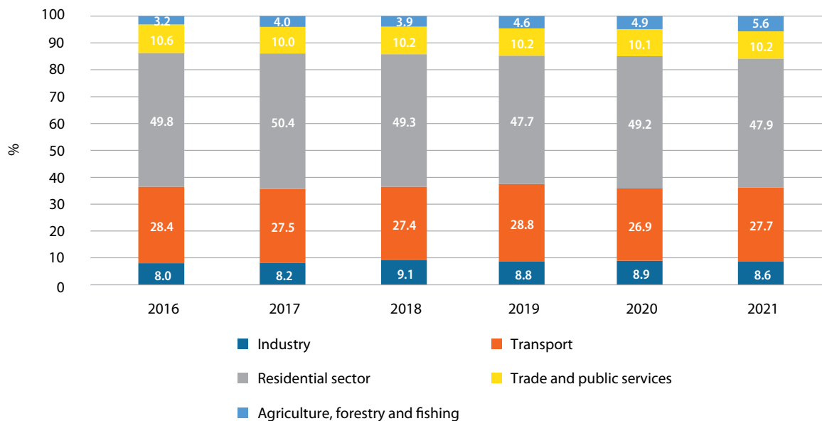
Figure 3 Final energy consumption by sector for 2016-2021 (%)
